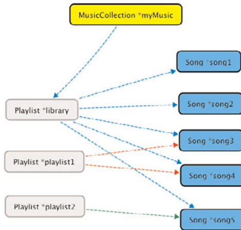
Figure 15.6 Example music collection data structures
