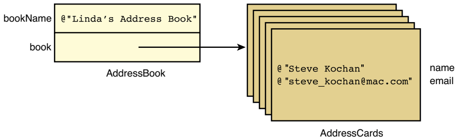
Figure 15.5 An AddressBook that contains AddressCards
