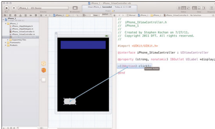
Figure 21.15 Adding an action for a button
