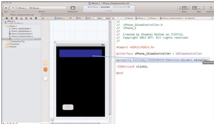
Figure 21.16 Connecting an outlet variable
