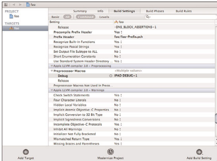
Figure 12.1 Defining the preprocessor identifier IPAD
