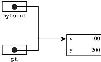
Figure 8.6 Passing the rectangle's origin to the method
