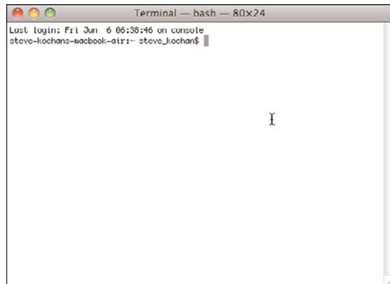
Figure 2.11 Terminal window
