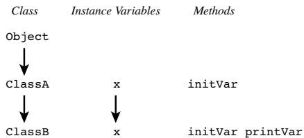
Figure 8.9 Overriding the initVar method
