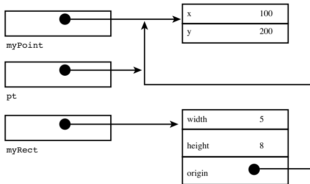
Figure 8.7 Setting the rectangle's origin
