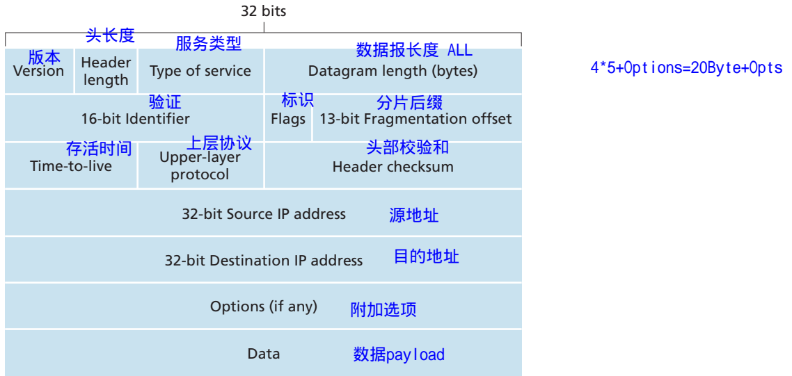
Figure 4.13 ♦ IPv4 datagram format
