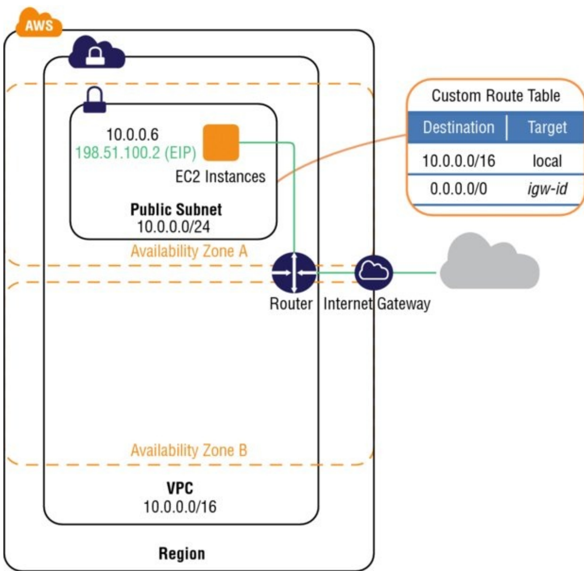
FIGURE 4.2 VPC, subnet, route table, and an Internet gateway
