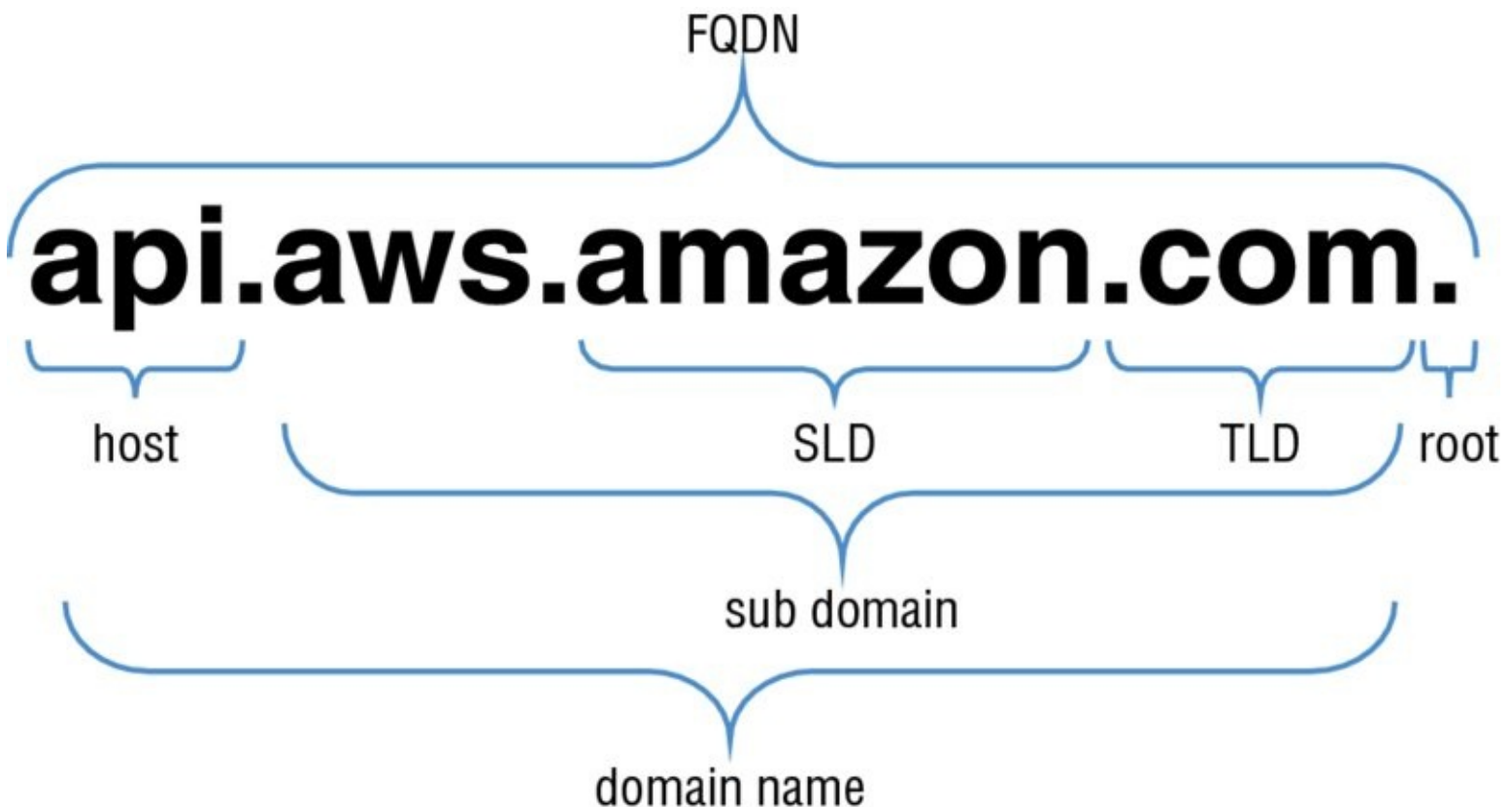
FIGURE 9.1 FQDN components
