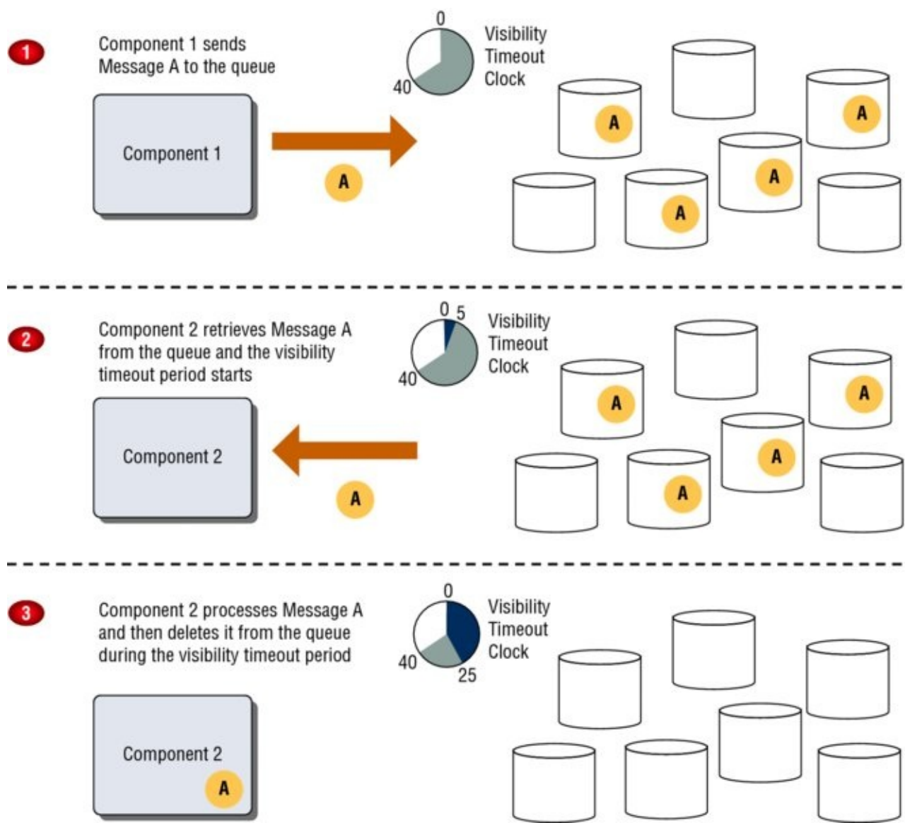
FIGURE 8.1 Message lifecycle
