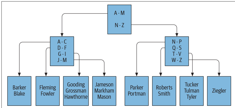
Figure 13-1. B-tree example
