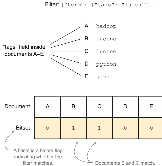
Figure 4.3 Filter results are cached in bitsets, making subsequent runs much faster.
