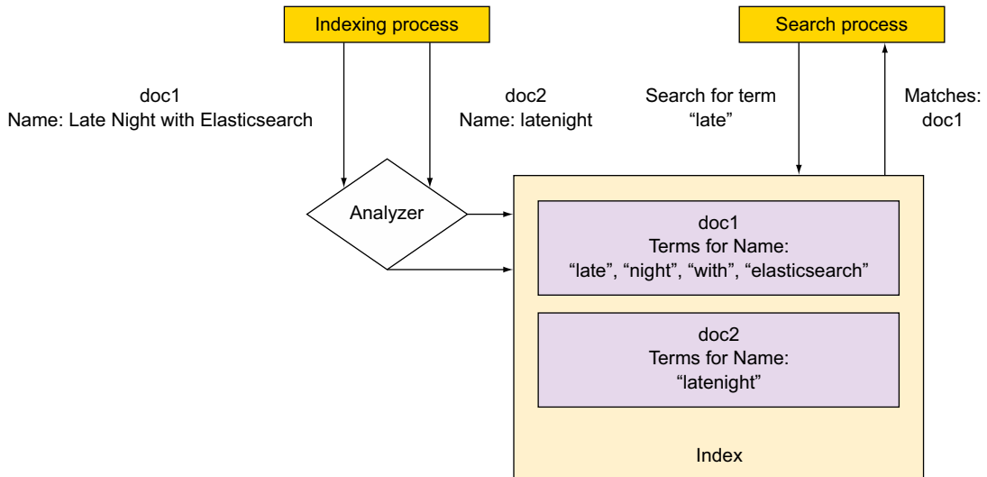
Figure 3.2 After the default analyzer breaks strings into terms, subsequent searches match those terms.
