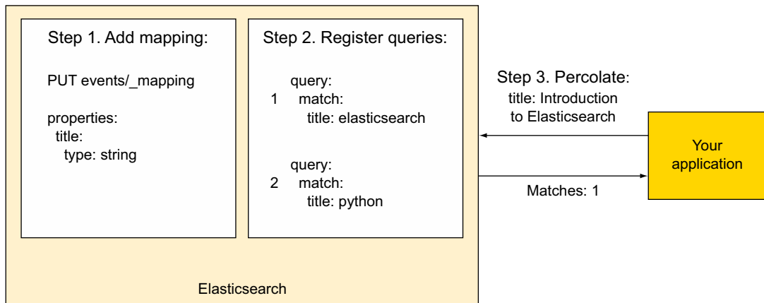
Figure E.2 You need a mapping and some registered queries in order to percolate documents.
