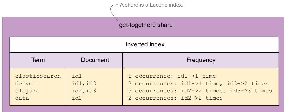
Figure 2.5 Term dictionary and frequencies in a Lucene index
