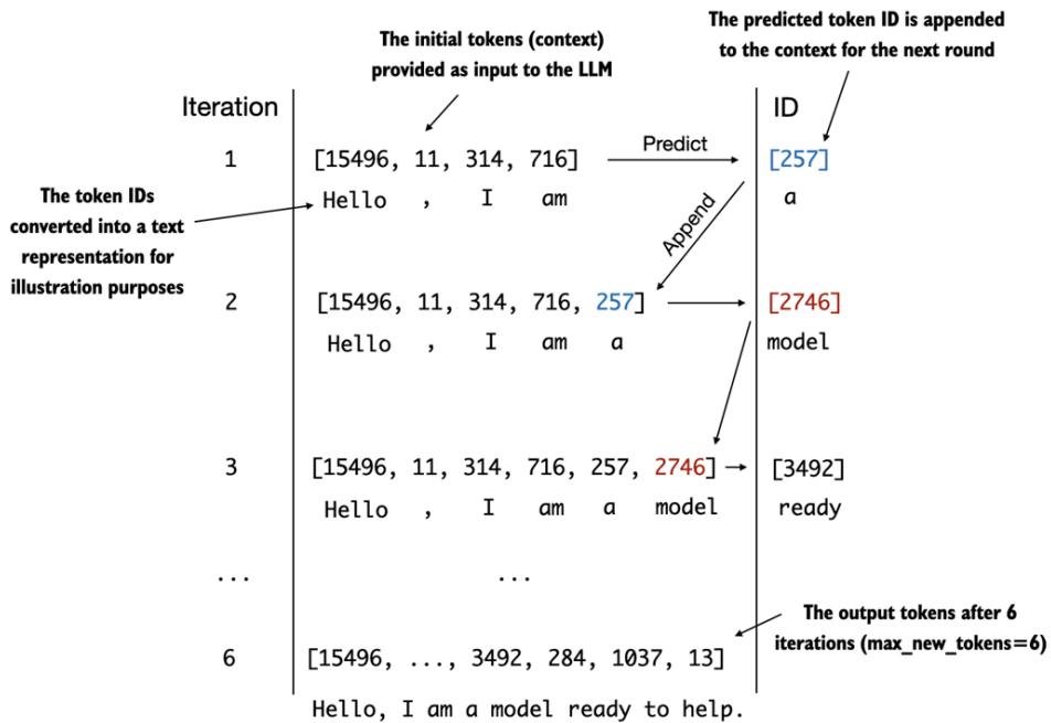
Figure 4.18 An illustration showing six iterations of a token prediction cycle, where the model takes a sequence of initial token IDs as input, predicts the next token, and appends this token to the input sequence for the next iteration. (The token IDs are also translated into their corresponding text for better understanding.)
