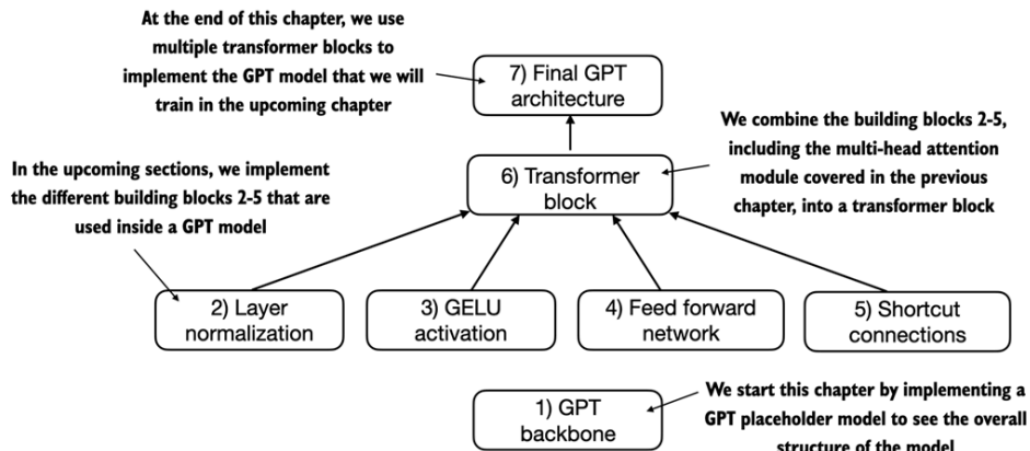
Figure 4.3 A mental model outlining the order in which we code the GPT architecture. In this chapter, we will start with the GPT backbone, a placeholder architecture, before we get to the individual core pieces and eventually assemble them in a transformer block for the final GPT architecture.
